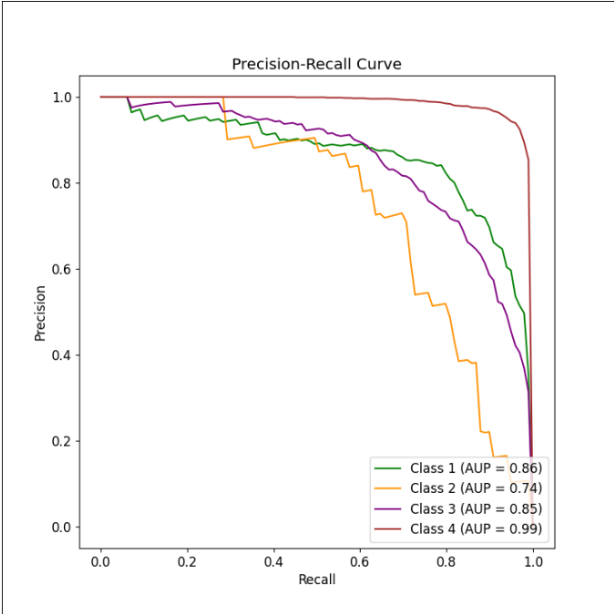
PR curve
