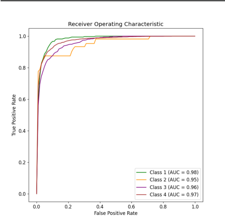
ROC curve
